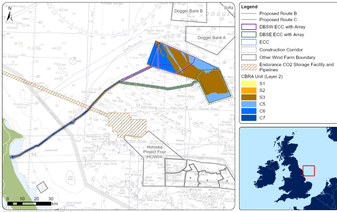
Figure 12: GM CBRA model geological units (Layer 2)
