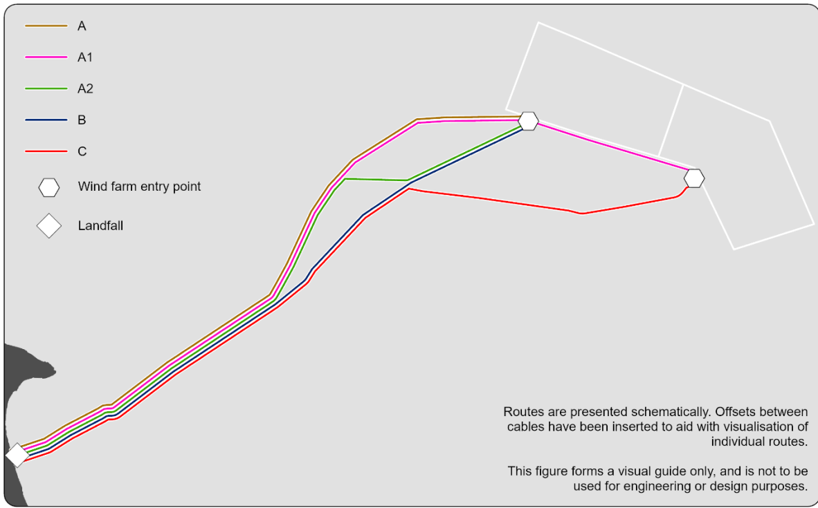
Figure 3: Initial cable route options schematic
